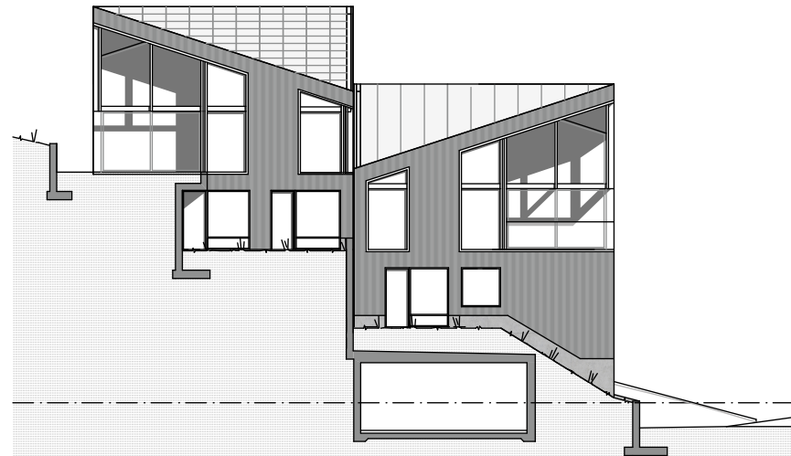
FASSADE WEST
